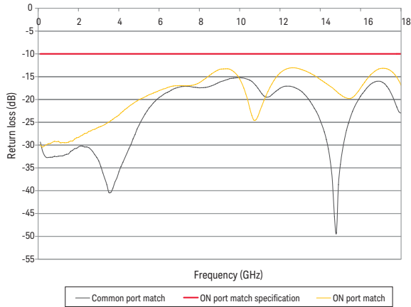
Figure 9. P9402C return loss (ON) vs. frequency (typical)
