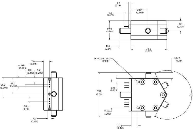
Figure 3. Product dimensions for P9404A/C
