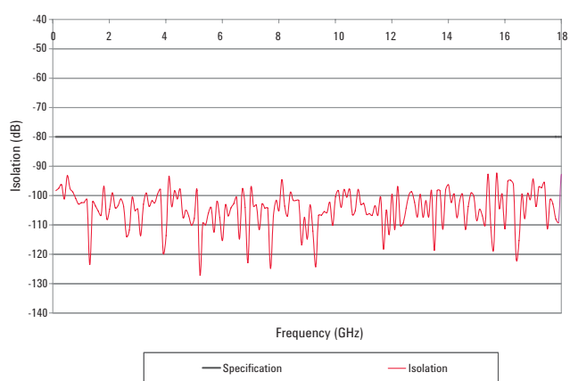
Figure 19. P9404C isolation vs. frequency (typical)
