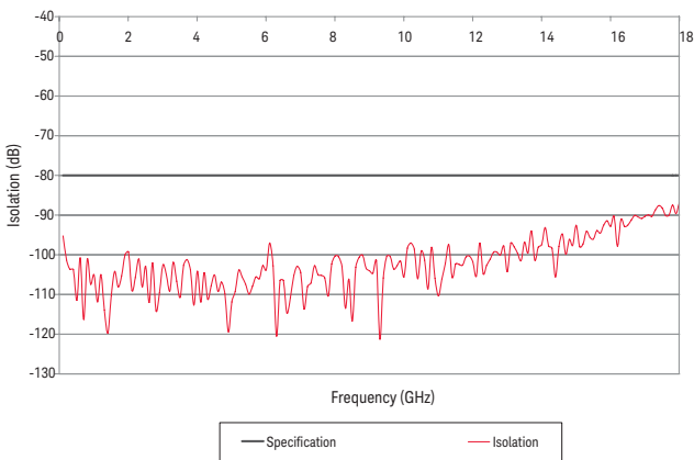
Figure 11. P9402C isolation vs. frequency (typical)
