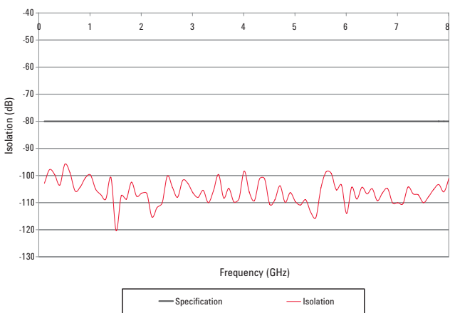
Figure 15. P9404A isolation vs. frequency (typical)
