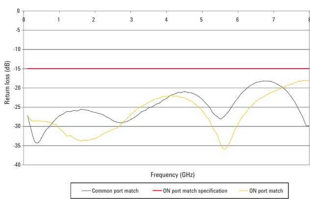
Figure 13. P9404A return loss (ON) vs. frequency (typical)
