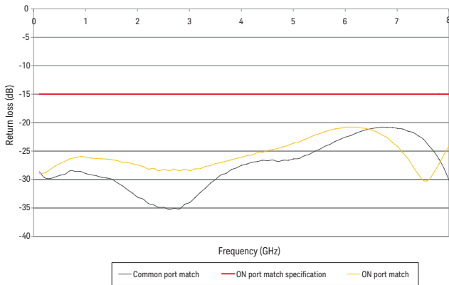
Figure 5. P9402A return loss (ON) vs. frequency (typical)
