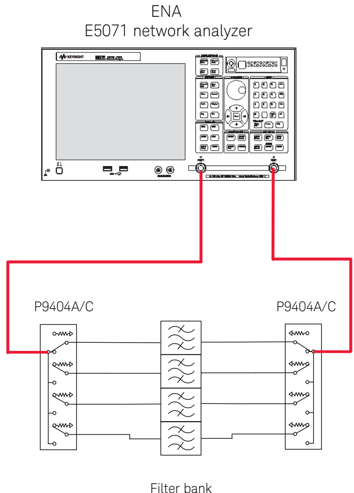
Figure 1. Filter bank test setup
