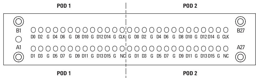
Figure 3.12. Pinout
