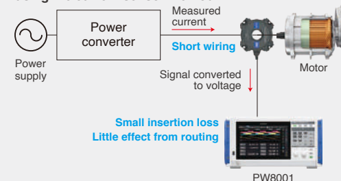
Measurement example using the current sensor method
