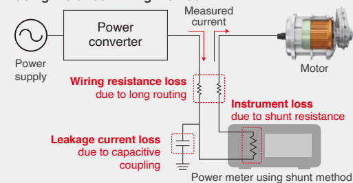
Measurement example using the direct wiring method
